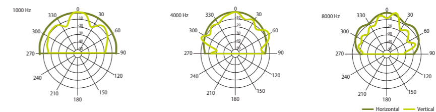
HORIZONTAL / VERTICAL POLAR DIAGRAMS
