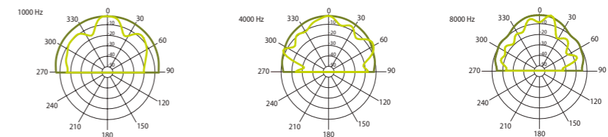
HORIZONTAL / VERTICAL POLAR DIAGRAMS
