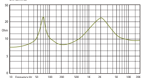
IMPEDANCE
