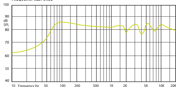
FREQUENCY RESPONSE
