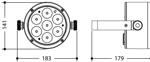
Technical drawing
