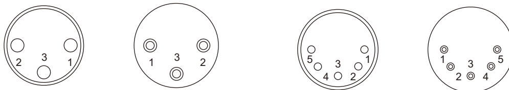
3 pin XLR
