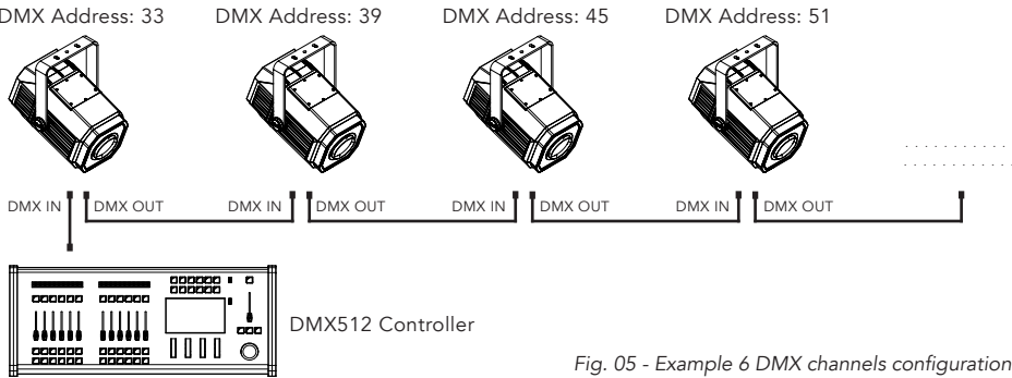
Fig. 05 - Example 6 DMX channels configuration
