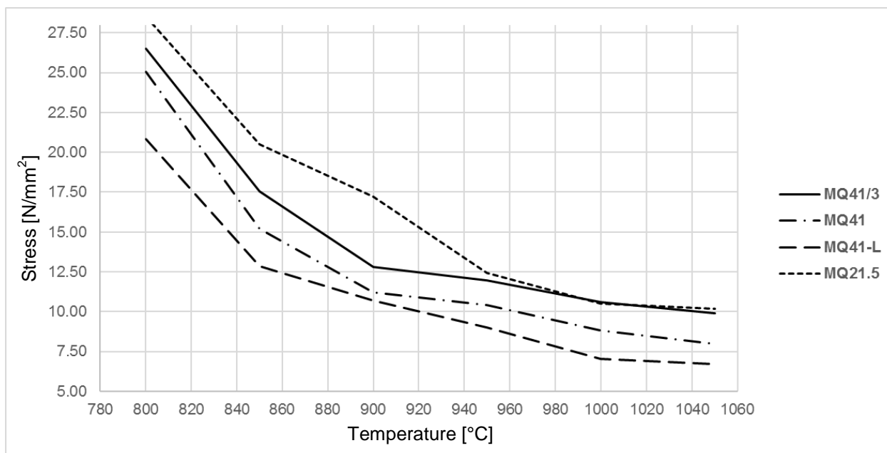
Figure D2: Channel material stress at 2% strain
