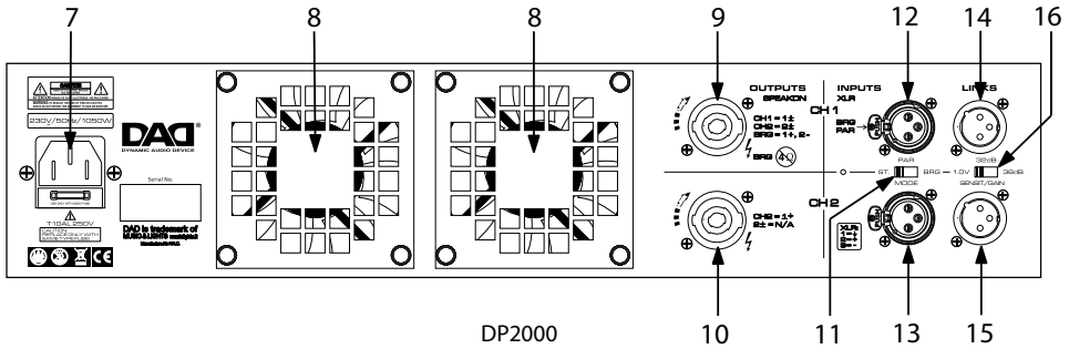
Pannello posteriore - Rear panel
