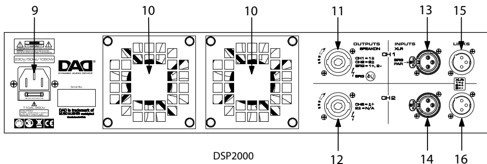
Pannello posteriore - Rear panel
