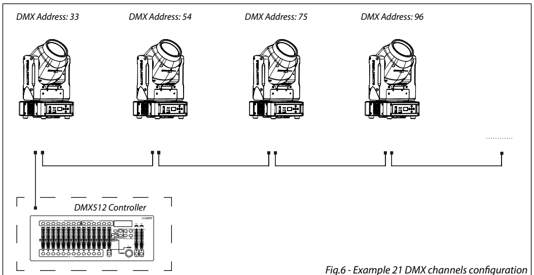
Fig.6 - Example 21 DMX channels configuration
