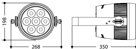
Technical drawing
