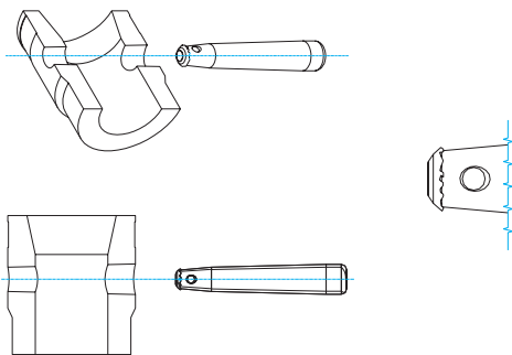
Deformation of the conical pins
