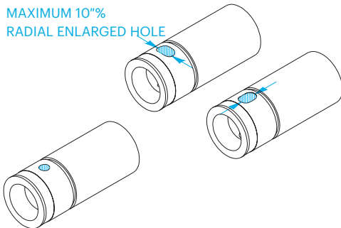
Enlargement of the conical drill holes
