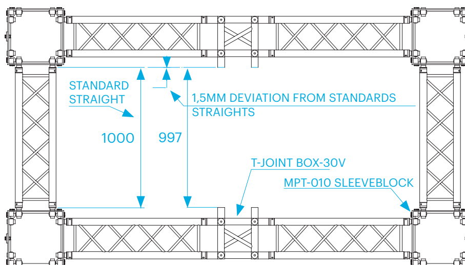
Combination of BOX-30V and MPT-010
