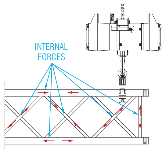
Normal force in a truss
