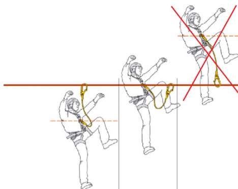
Fall arrest system with shock absorber
