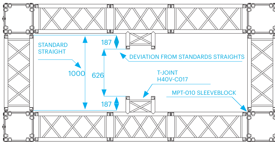
Combination of H40V-C017 and MPT-010
