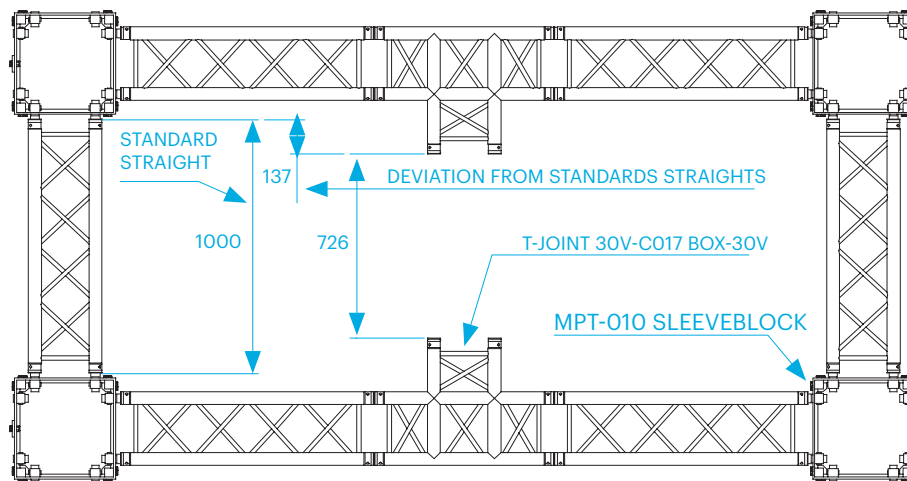
Combination of H30V-C017 and MPT-010
