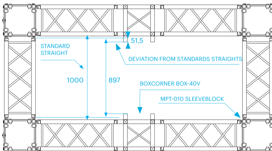
Combination of BOX-40V and MPT-010
