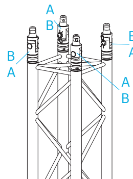
A = CCS6-H-FM-45° B = CCS6-H-M-135°
