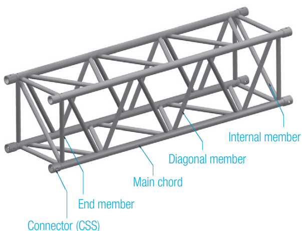
Elements of a truss
