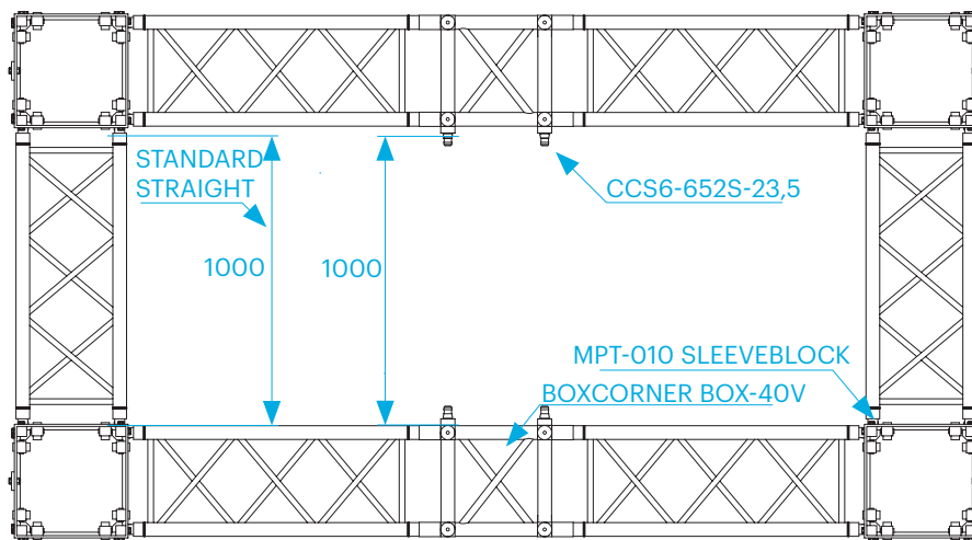
Combination of BOX-40V with CCS6-652S-23,5 and MPT-010
