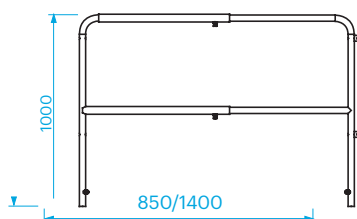
EasyRail railing. SM-RAIL-L85/140.
